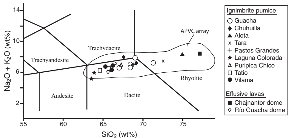
Figure 5. Total alkalis versus silica diagram of pumice from Bolivian ignimbrites and lavas analyzed in this study. Also shown is array of Altiplano-Puna volcanic complex (APVC) ignimbrite pumice reported in de Silva (1987), Lindsay et al. (2001b), Ort et al. (1996), and Soler et al. (2007). Altiplano-Puna volcanic complex ignimbrites and lavas are dominantly dacitic with lesser volumes of rhyolite.
