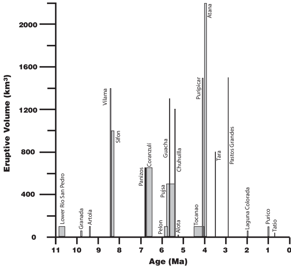
Figure 8. Volume-time relations of Altiplano-Puna volcanic complex ignimbrites. Horizontal width of each unit is ±2σ of the preferred age of each unit listed in Table 5.
